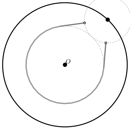
FIGURE 1.1. An example where M = \partial B_R(O) , where R > 4.98r .
