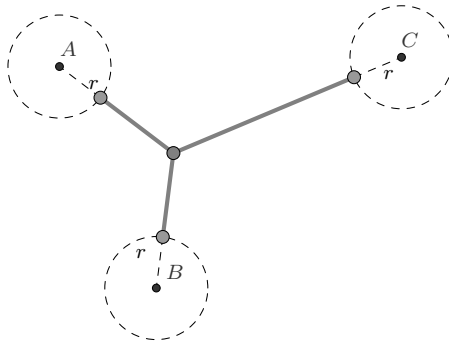
FIGURE 1.3. An example where M := \{A, B, C\} , \Sigma is a tripod.
