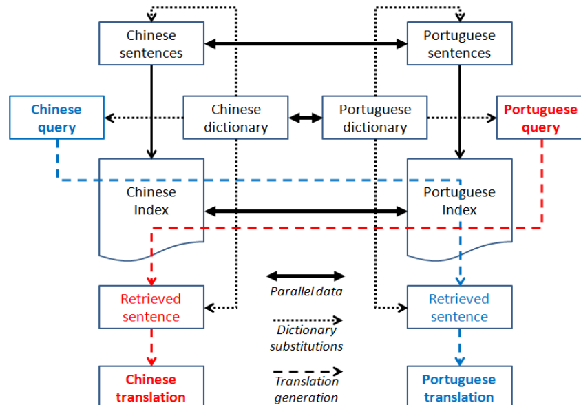
Fig. 2. Proposed approach for off-line translation by means of an information retrieval strategy over the collection of the most commonly requested translation pairs.
